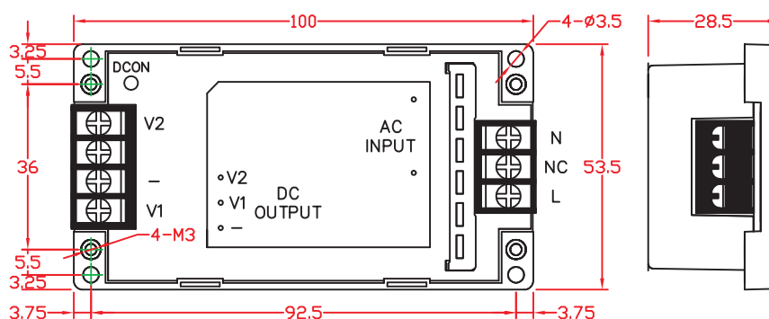
Standard Mountable
