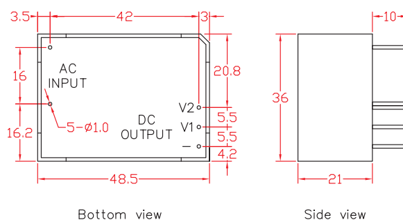
PCB Mountable
